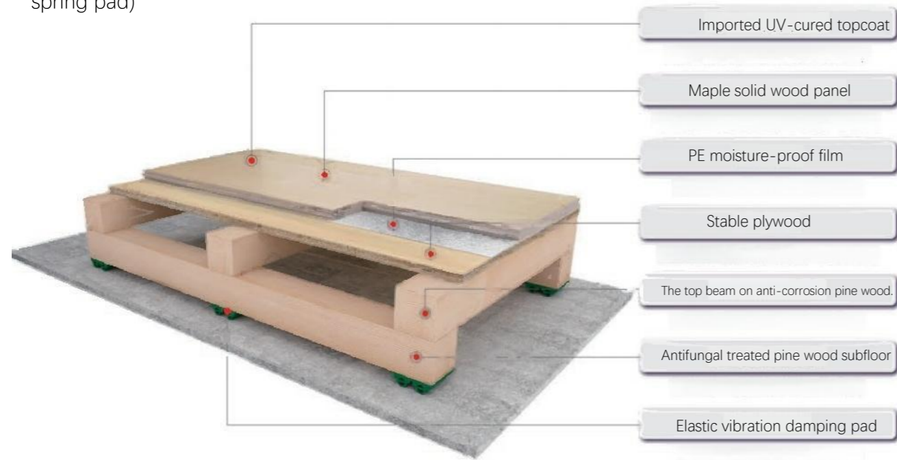
Double-layered batten structure system (single spring pad/double spring pad)
