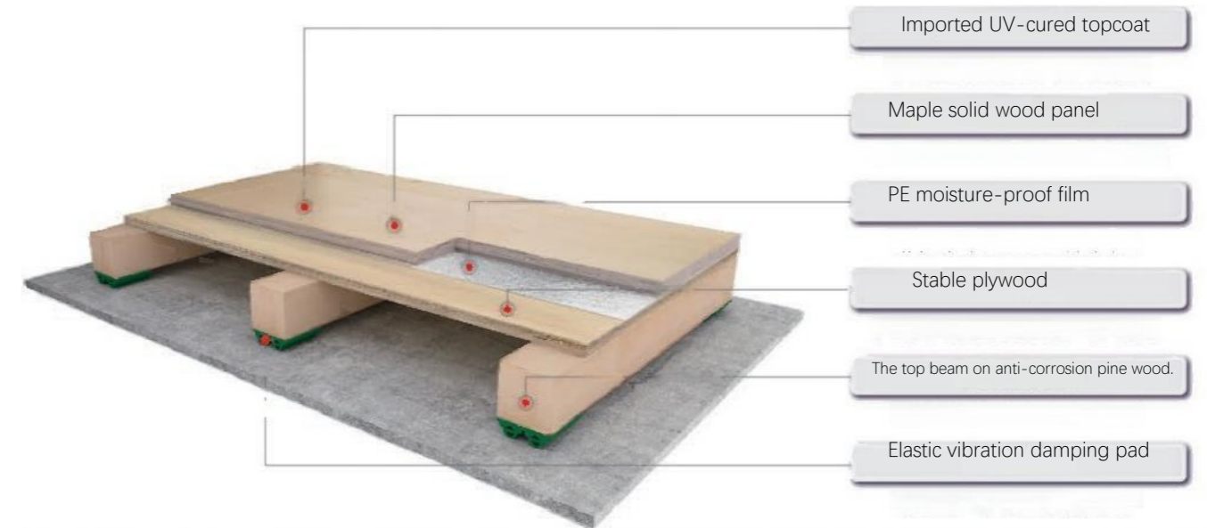
Single-layer batten structure system
